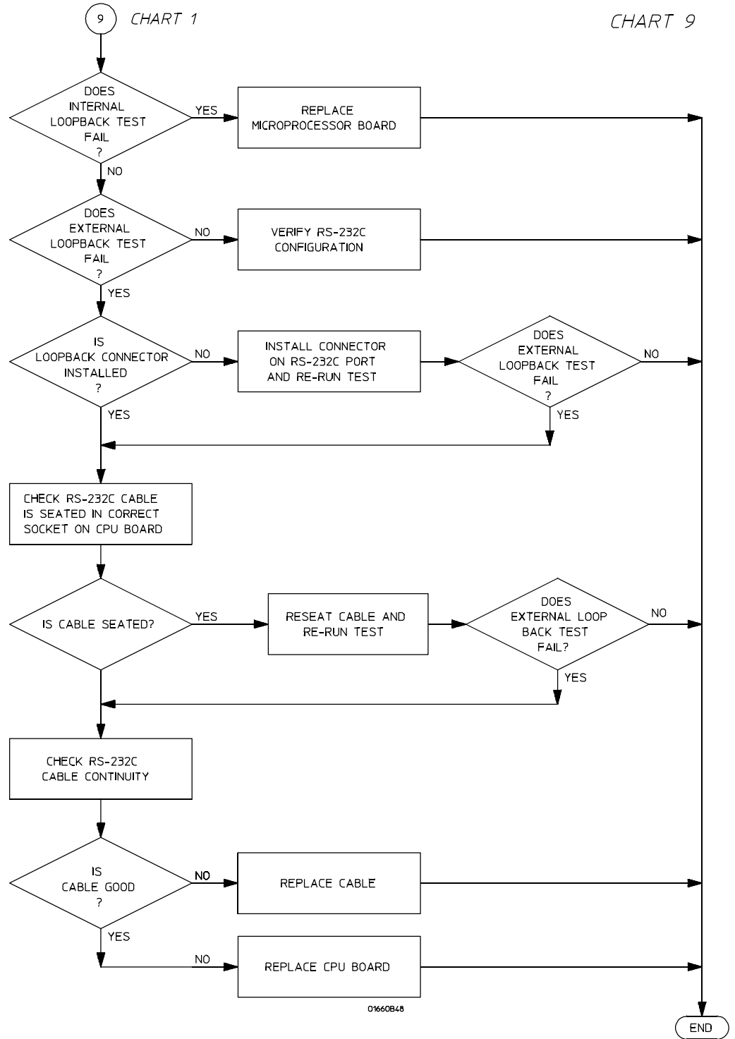
Troubleshooting Flowchart 9
